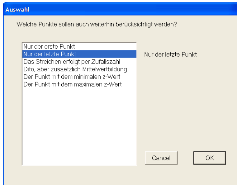
Abbildung 3-32: Pcgdoubl-Fenster
